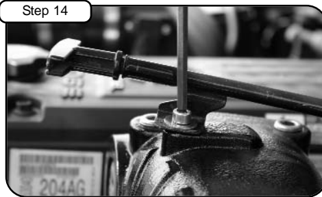
Step 14 Install the engine oil dipstick using M6 fender washer and socket cap screw provided. Tighten using 5mm allen key (See notes 1, 2 & 3). Attach the engine wire harness to the aFe manifold.
